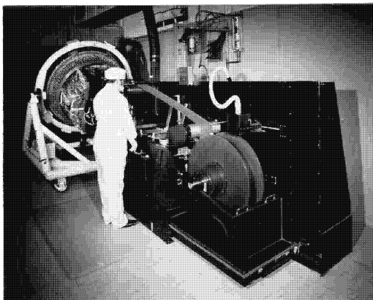
Figure 22 - Hexagon SRV Interfaced with Presplice Complex
