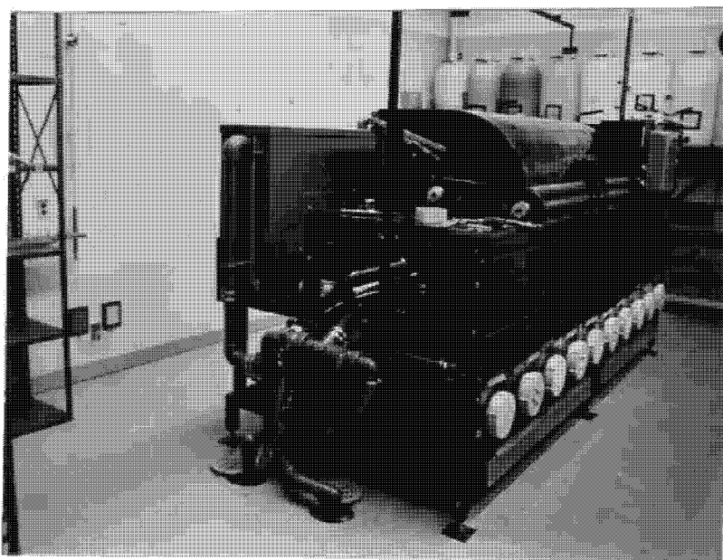
Figure 58 - Automat Processor
