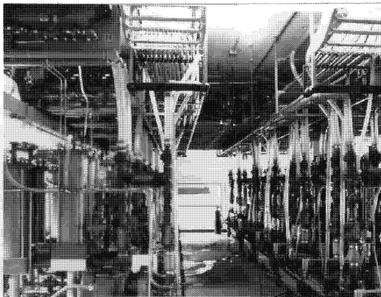
Figure 51 - (MP) 2 Mezzanine
