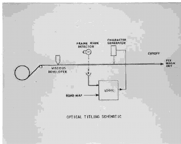
Figure 27 - Optical Titling Schematic.
